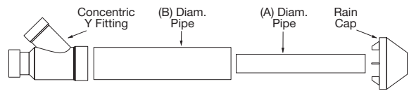
2", 3" and 4" Concentric Vent Kits Part Identification
